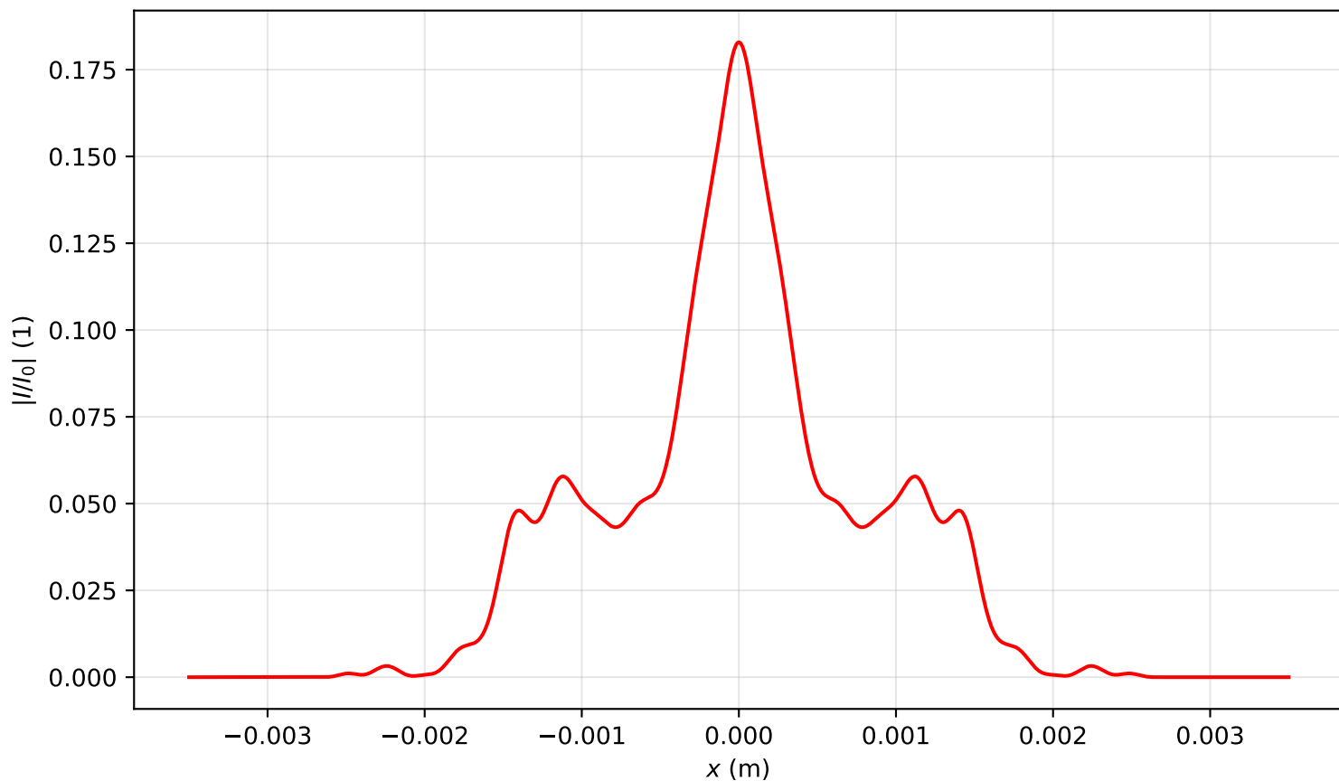
Intensity profile I(x, y = 0, z = 3.105)/I_0 , P_{in}=5.5P_{cr} , artificial time
